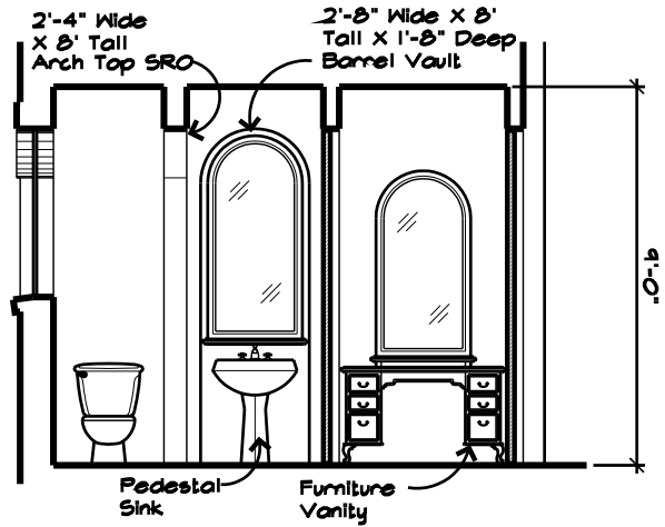
POWDER ELEVATION 3/8" = 1'-0"
